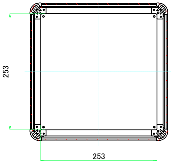
C-C (1:5)
