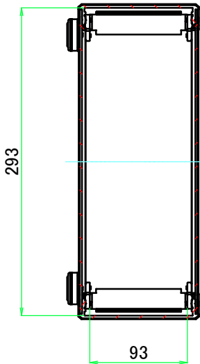
B-B (1:5)
